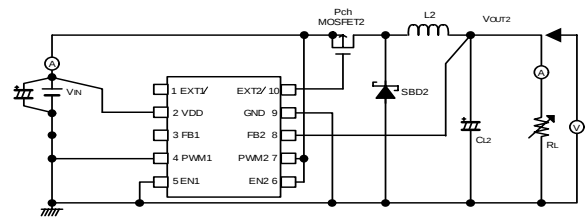
Circuit 7
