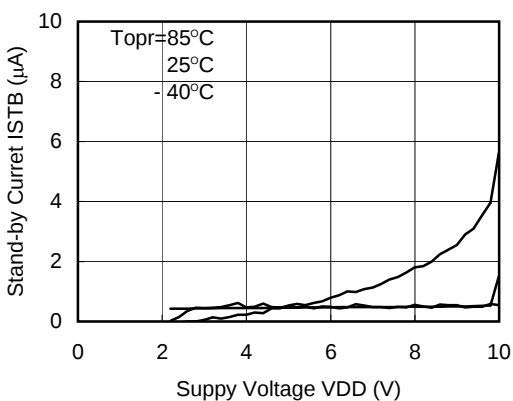
XC9503B092 (180KHz)
