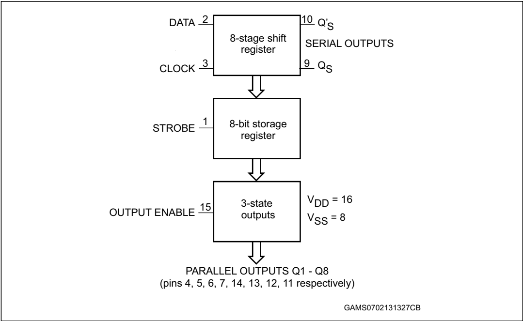
Figure 3. Functional diagram
