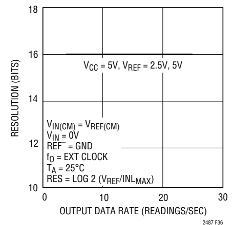
Figure 36. Resolution ( \text{INL}_{\text{MAX}} \leq 1\text{LSB} ) vs Output Data Rate and Temperature
