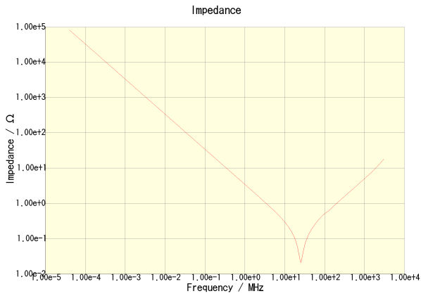
C2012X7R2A473K125AA
