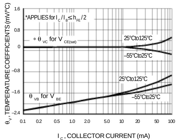
Figure 11. Temperature Coefficients
