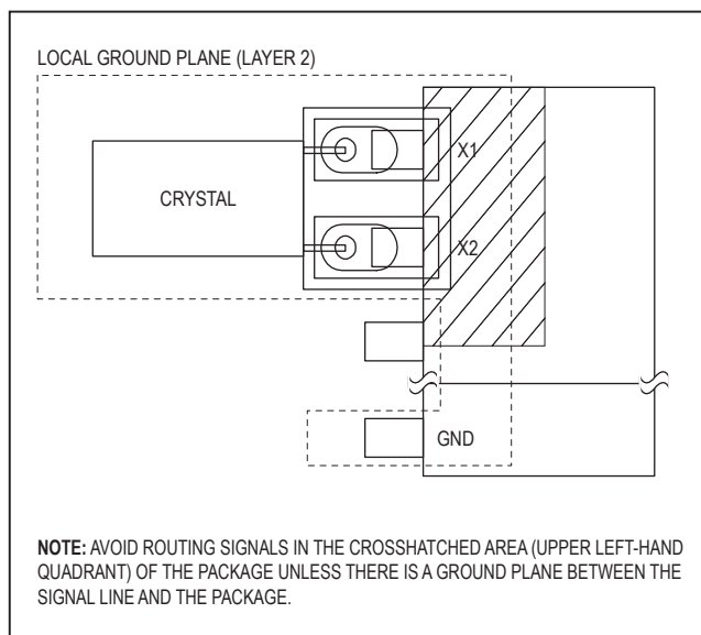
Figure 2. Layout Example
