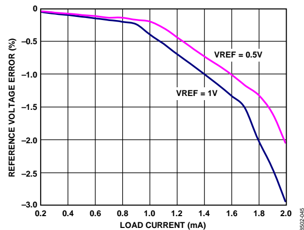
If the internal reference of the AD9265 is used to drive multiple converters to improve gain matching, the loading of the reference by the other converters must be considered. Figure 72 shows how the internal reference voltage is affected by loading.
