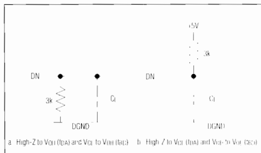
Figure 1. Load Circuits for Access Time
