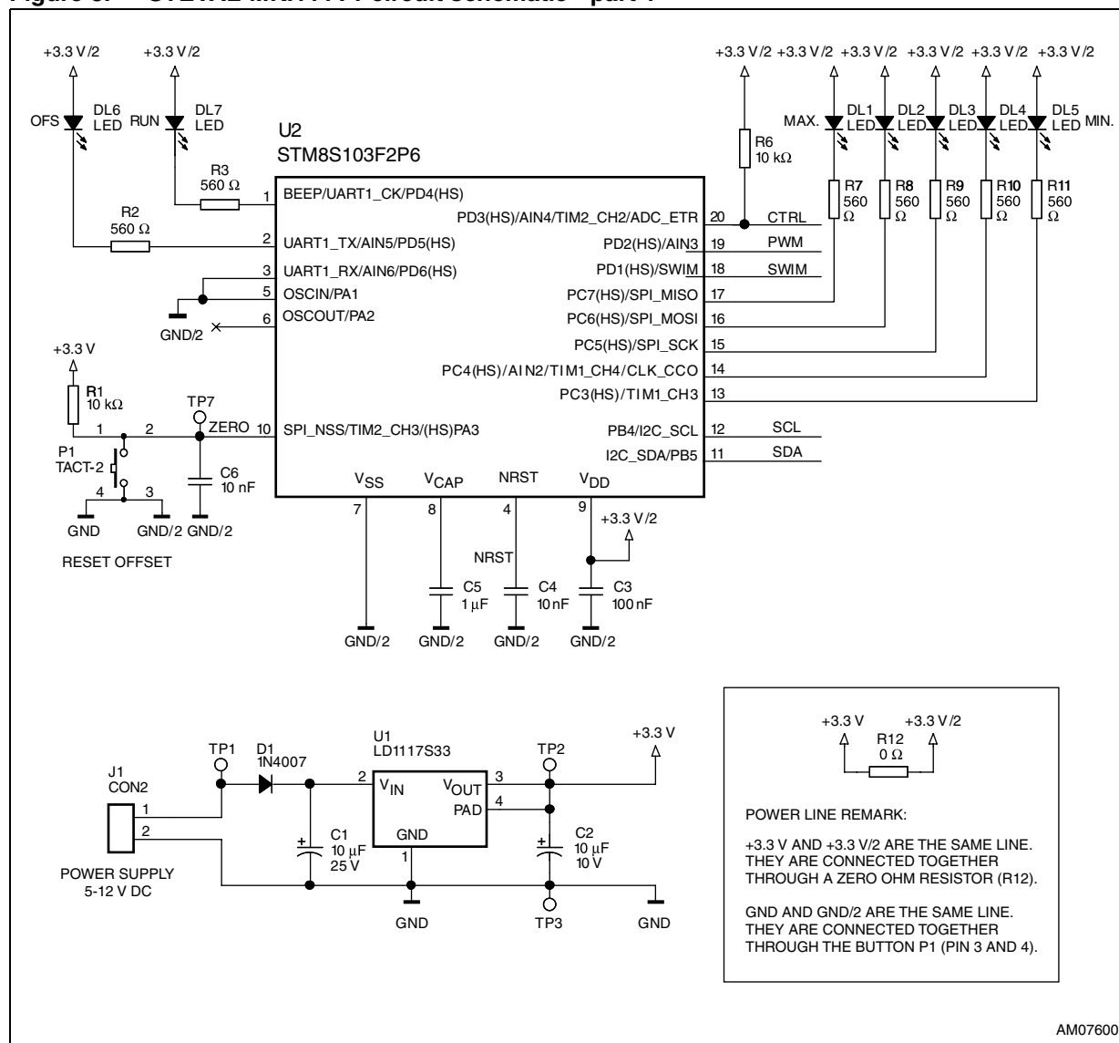
Figure 3. STEVAL-MKI111V1 circuit schematic - part 1
