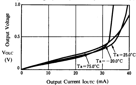
Output Voltage ( V_{OLC} ) vs. Output Current ( I_{OUTC} )
