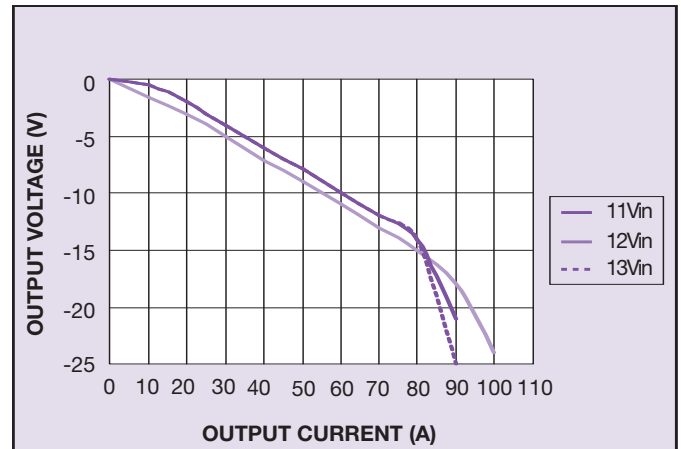
Figure 2: Load Regulation
