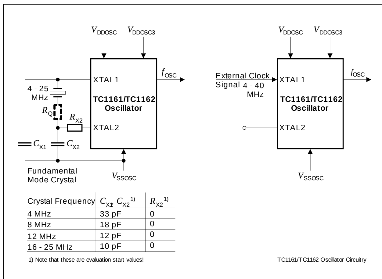
Figure 3-15 Oscillator Circuitries
