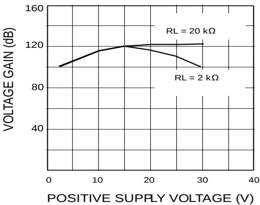
Figure 12: Open-loop gain
