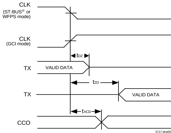
Figure 9. Serial Output and External Control
