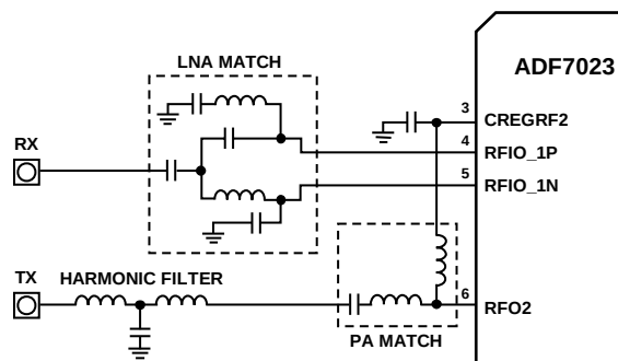
Figure 114. Separate Single-Ended PA and LNA Match
