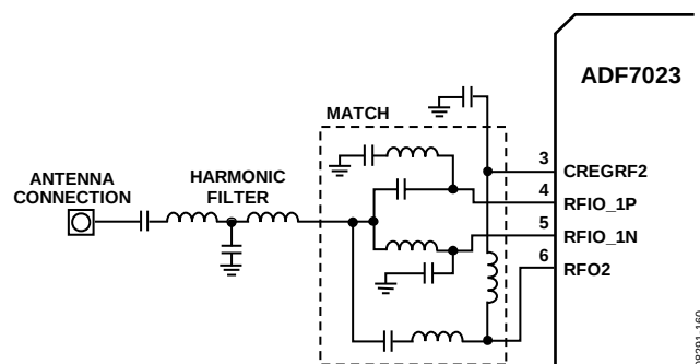
Figure 113. Combined Single-Ended PA and LNA Match
