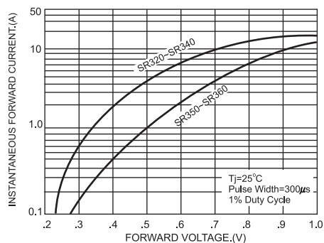
FIG.2-TYPICAL FORWARD CHARACTERISTICS
