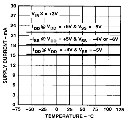
Figure 19. Supply Current vs. Supply Voltage vs. Temperature
