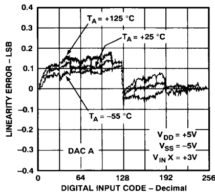
Figure 3. Linearity Error vs. Digital Code vs. Temperature
