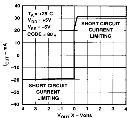
Figure 21. DAC Output Current vs. V_{OUTX}
