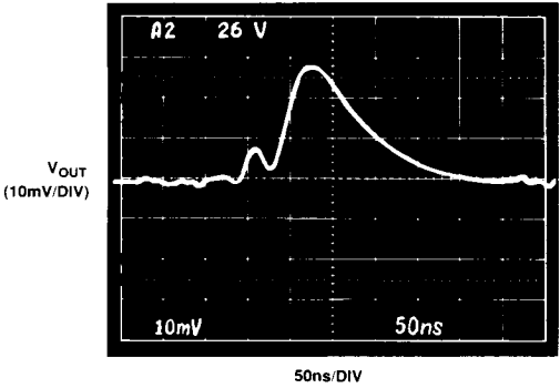
Figure 14. Digital Feedthrough
