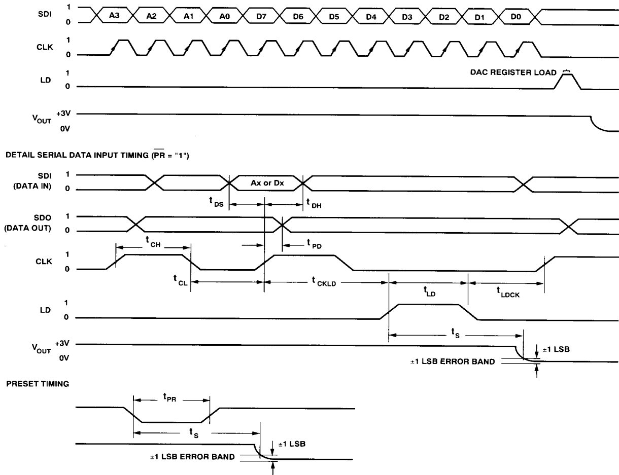
Figure 1. Timing Diagram
