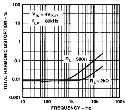
Figure 6. Total Harmonic Distortion vs. Frequency
