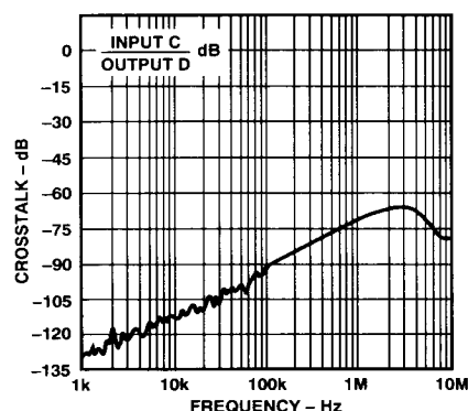
Figure 9. DAC Crosstalk vs. Frequency
