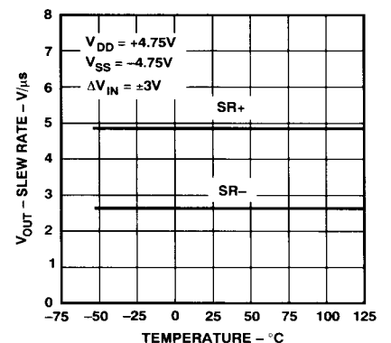
Figure 7. V_{OUT} Slew Rate vs. Temperature
