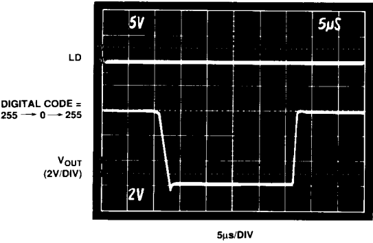
Figure 12. Settling Time
