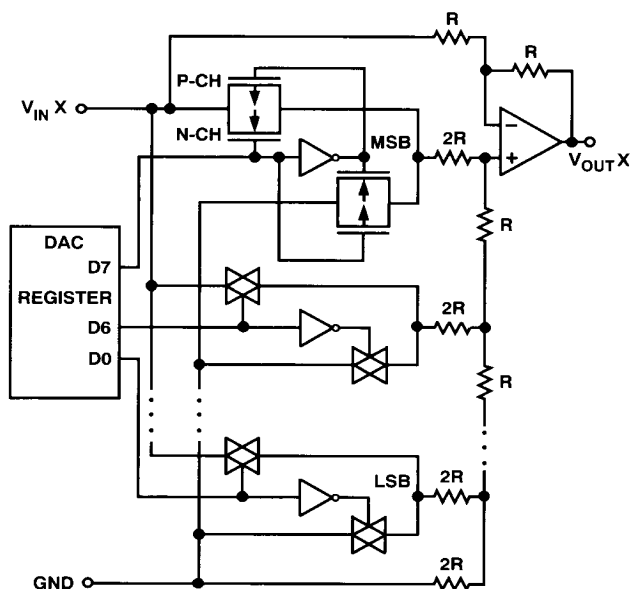
Figure 23. DAC-8840 TrimDAC Equivalent Circuit
