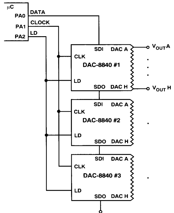
Figure 25. Three-Wire Interface Updates Multiple DAC-8840s
