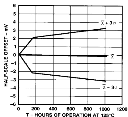
Figure 22. Output Drift Delta Accelerated by Burn-In
