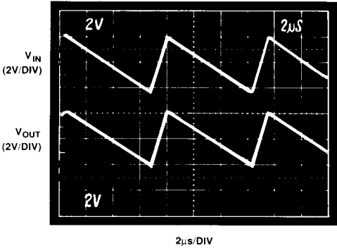
Figure 17. 128 kHz Sawtooth Waveform
