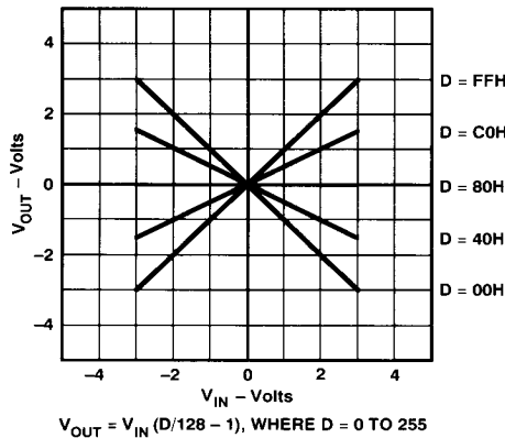
Figure 24. DAC Plus Amplifier Combine to Produce Four Quadrant Multiplication
