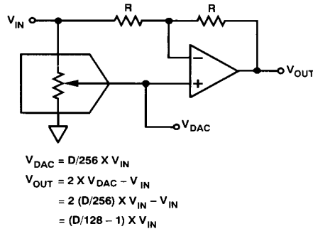
DAC8840 INPUT OUTPUT VOLTAGE RANGE
