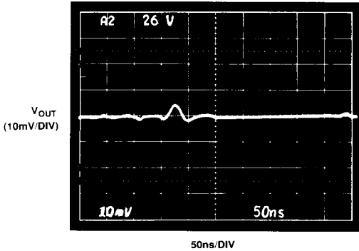
Figure 15. Digital Crosstalk
