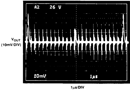
Figure 16. Clock Feedthrough
