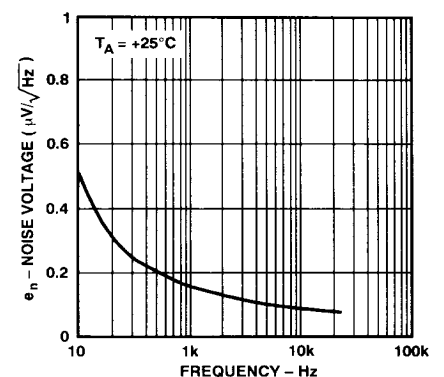
Figure 10. Voltage Noise Density vs. Frequency
