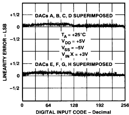
Figure 2. Linearity Error vs. Digital Input Code
