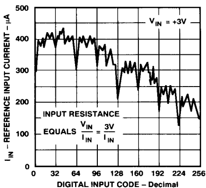
Figure 5. Input Resistance vs. Code
