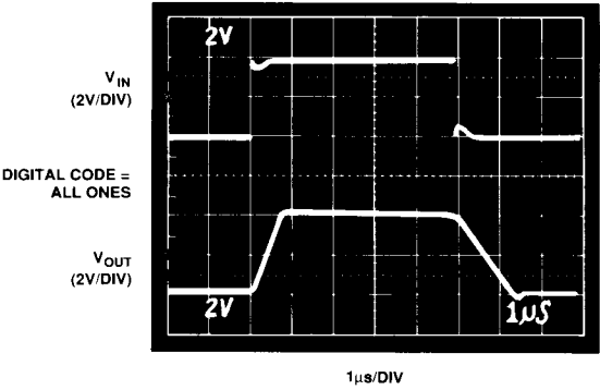
Figure 11. Pulse Response
