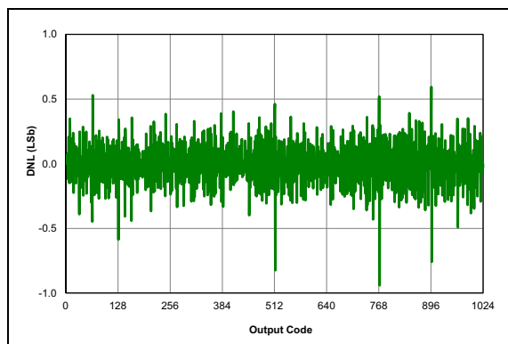
FIGURE 32-78: ADC 10-bit Mode, Single-Ended DNL, V_{DD} = 3.0V , T_{AD} = 4\text{ }\mu s , 25^\circ C .
