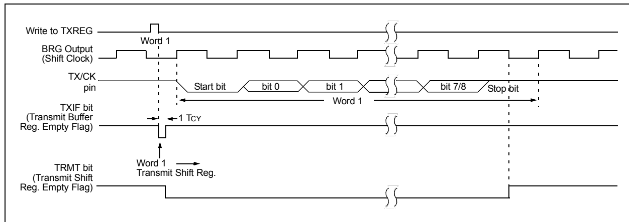
FIGURE 28-3: ASYNCHRONOUS TRANSMISSION
