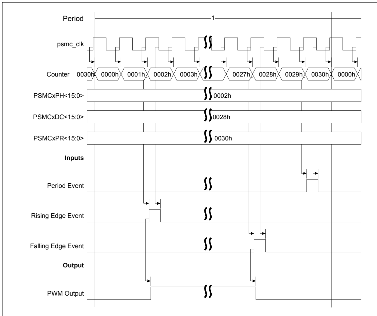
FIGURE 26-3: TIME BASE WAVEFORM GENERATION
