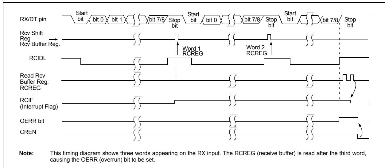
FIGURE 28-5: ASYNCHRONOUS RECEPTION
