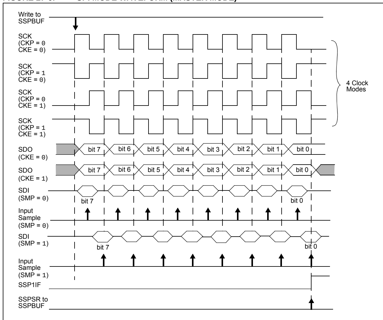
FIGURE 27-6: SPI MODE WAVEFORM (MASTER MODE)
