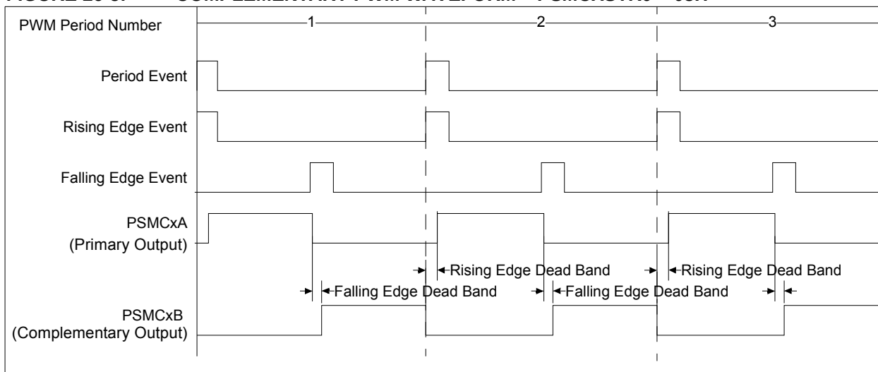
FIGURE 26-5: COMPLEMENTARY PWM WAVEFORM – PSMCXSTR0 = 03H
