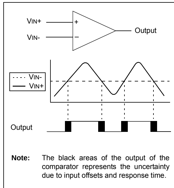
FIGURE 21-1: SINGLE COMPARATOR
