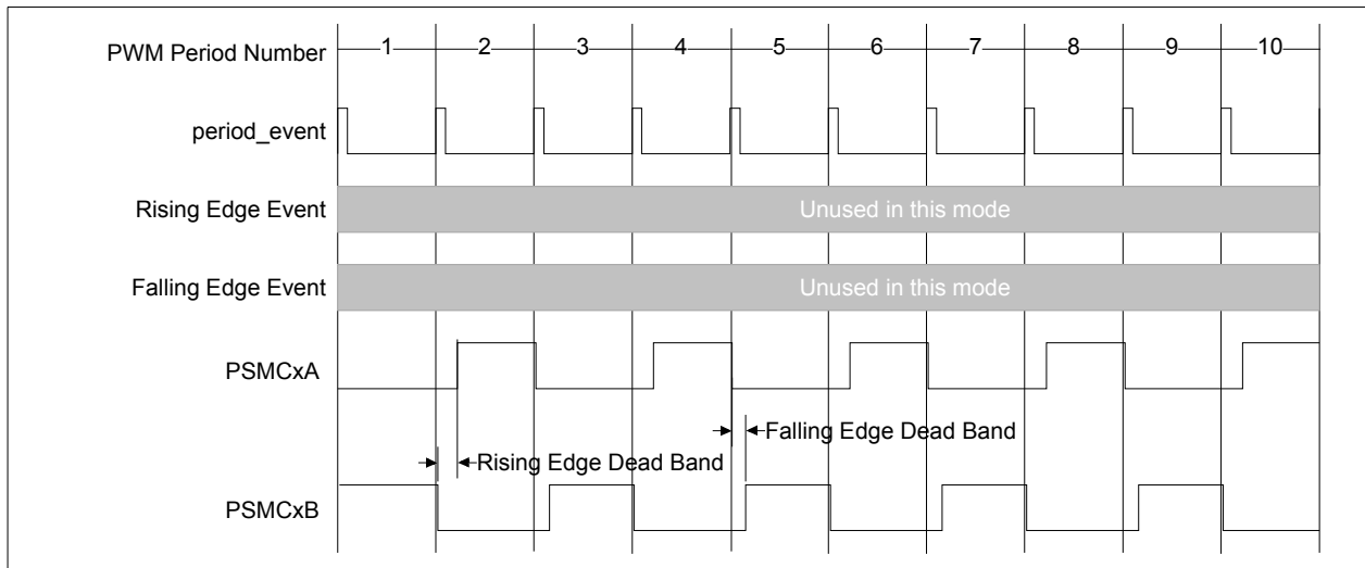
FIGURE 26-14: VARIABLE FREQUENCY – FIXED DUTY CYCLE PWM WITH COMPLEMENTARY OUTPUTS WAVEFORM
