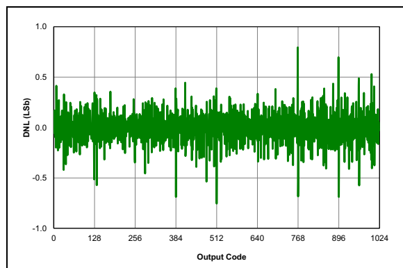
FIGURE 32-77: ADC 10-bit Mode, Single-Ended DNL, V_{DD} = 3.0V , T_{AD} = 1\text{ }\mu s , 25^\circ C .
