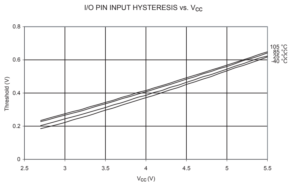
Figure 243. I/O Pin Input Hysteresis vs. V_{CC}
