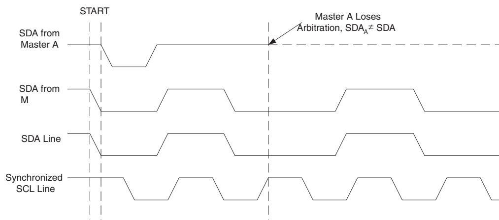
Figure 93. Arbitration between Two Masters
