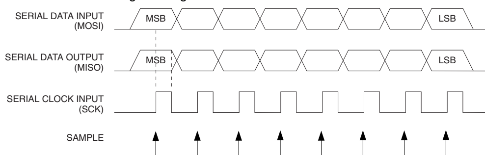
Figure 148. SPI Serial Programming Waveforms
