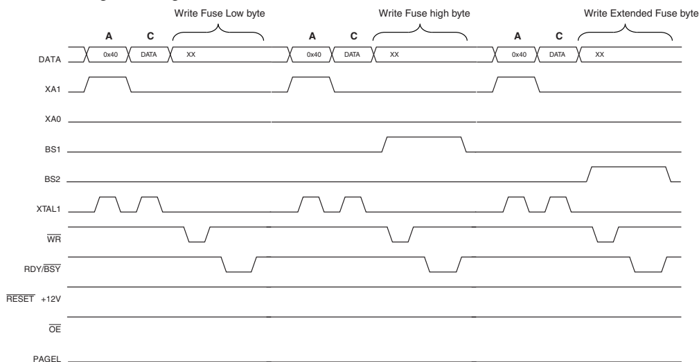
Figure 142. Programming the FUSES Waveforms
