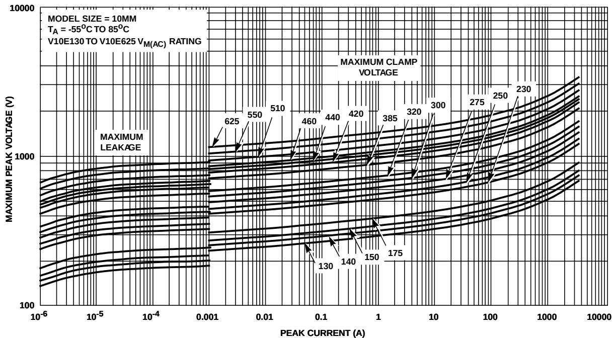
FIGURE 4. Clamping Voltage for VI10E130- V10E625
