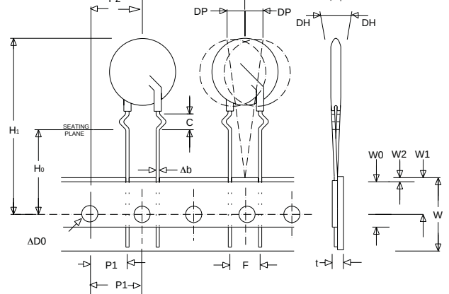
Crimped Leads "L2"
