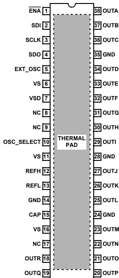
EL5525 (38-PIN HTSSOP) TOP VIEW
