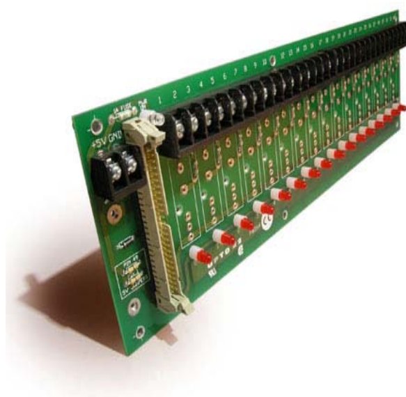
PB16H Rack
