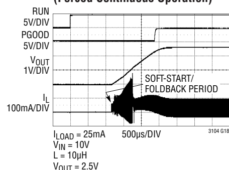
Start-Up from Shutdown (Forced Continuous Operation)
