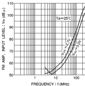
Fig. 2 FM amp input level vs. frequency characteristics
