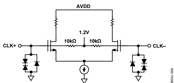
Figure 33. Clock Inputs
