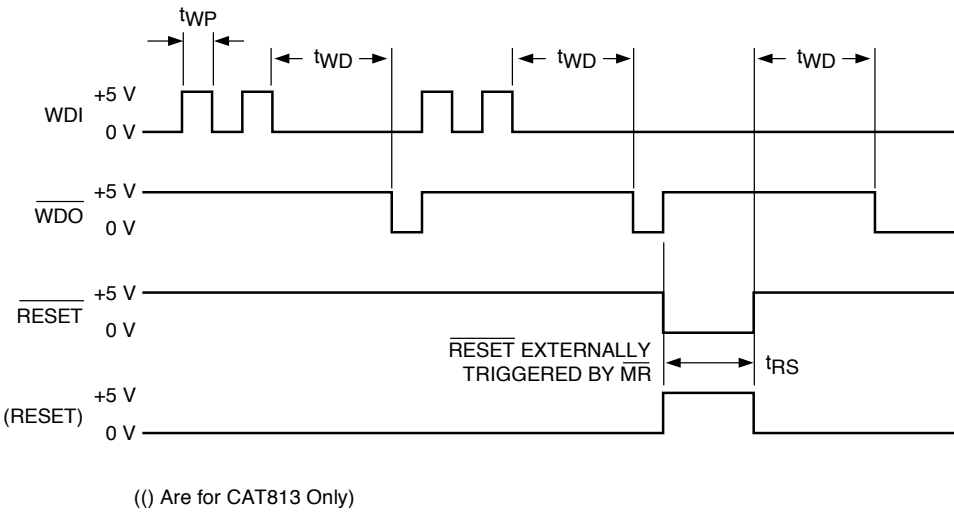
Figure 3. Watchdog Timing Diagram
