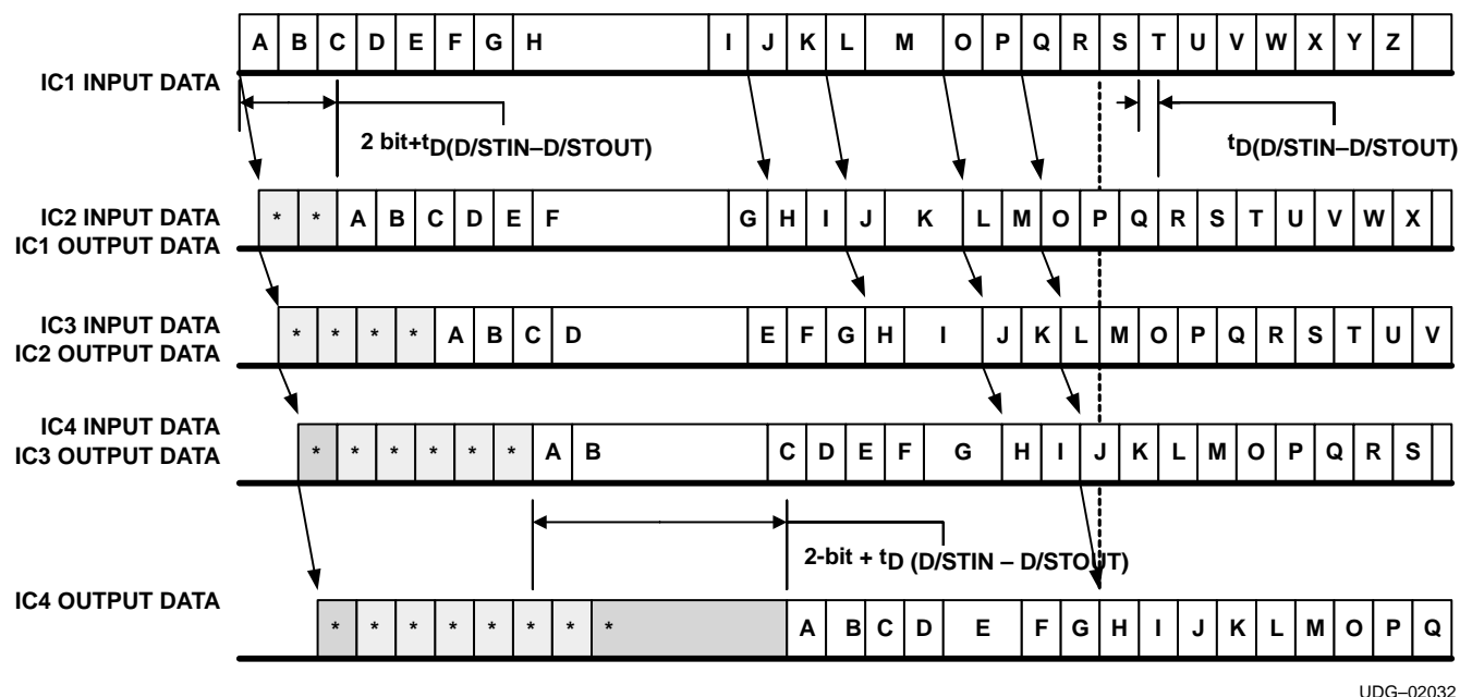
Figure 4. Data Transfer Concept in Cascade Connection
