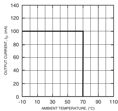
DERATING CHARACTERISTICS
