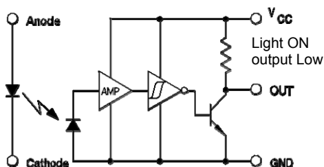
OPB916I Inverted 10K Pull-Up
