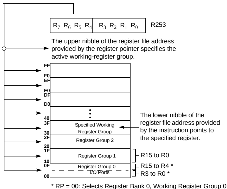
Figure 14. Register Pointer—Detail
