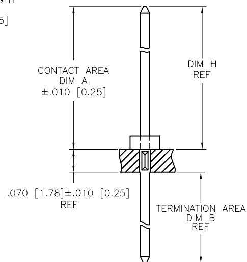
SECTION THRU PC BOARD SCALE 2:1
