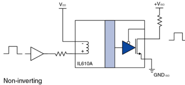
Non-inverting
