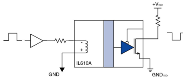
Inverting
