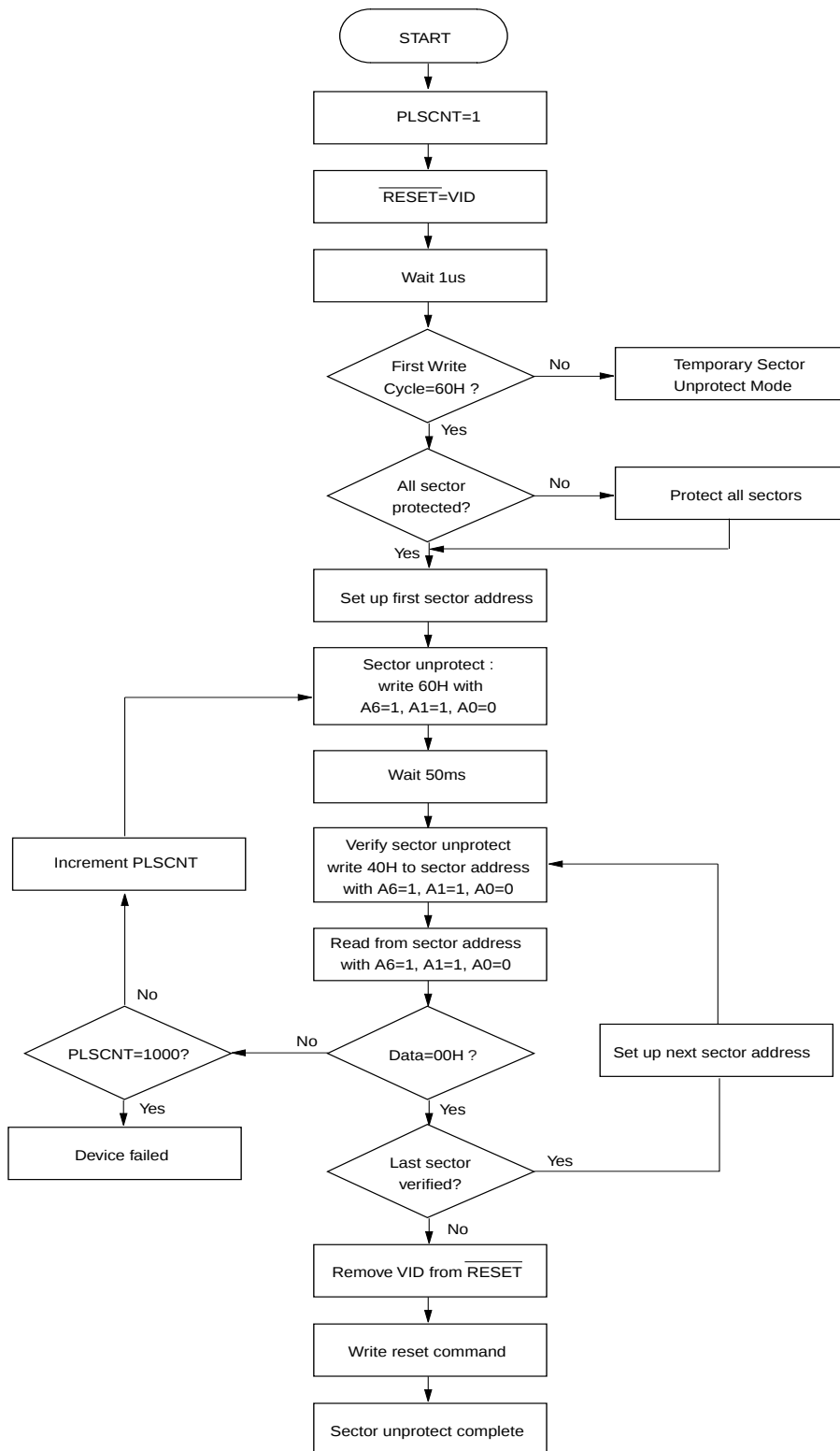
Figure 15. IN-SYSTEM CHIP UNPROTECTION ALGORITHM WITH \overline{\text{RESET}}=\text{VID}
