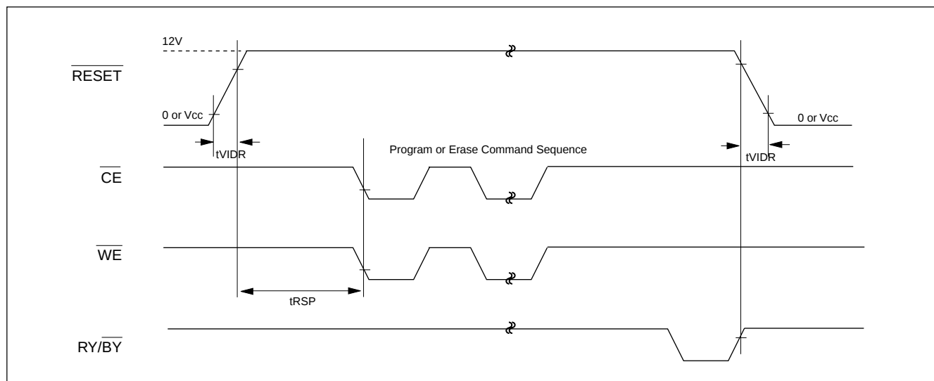
Figure 26. TEMPORARY SECTOR UNPROTECT TIMING DIAGRAM
