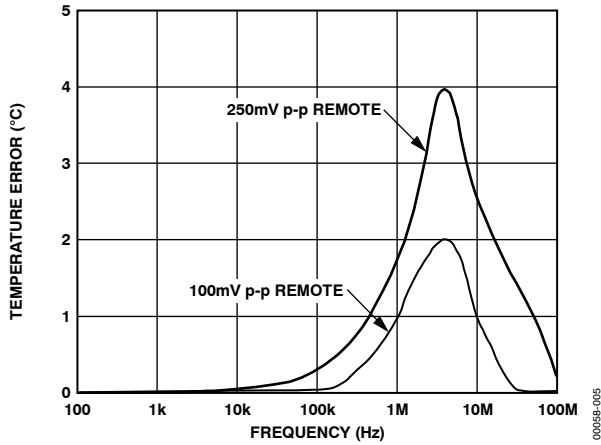
Figure 5. Remote Temperature Error vs. Supply Noise Frequency
