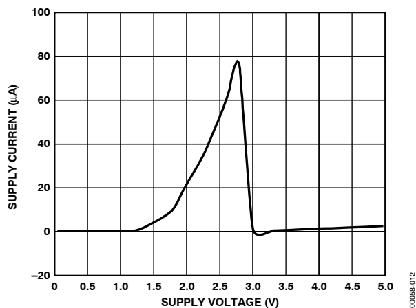
Figure 12. Standby Supply Current vs. Supply Voltage
