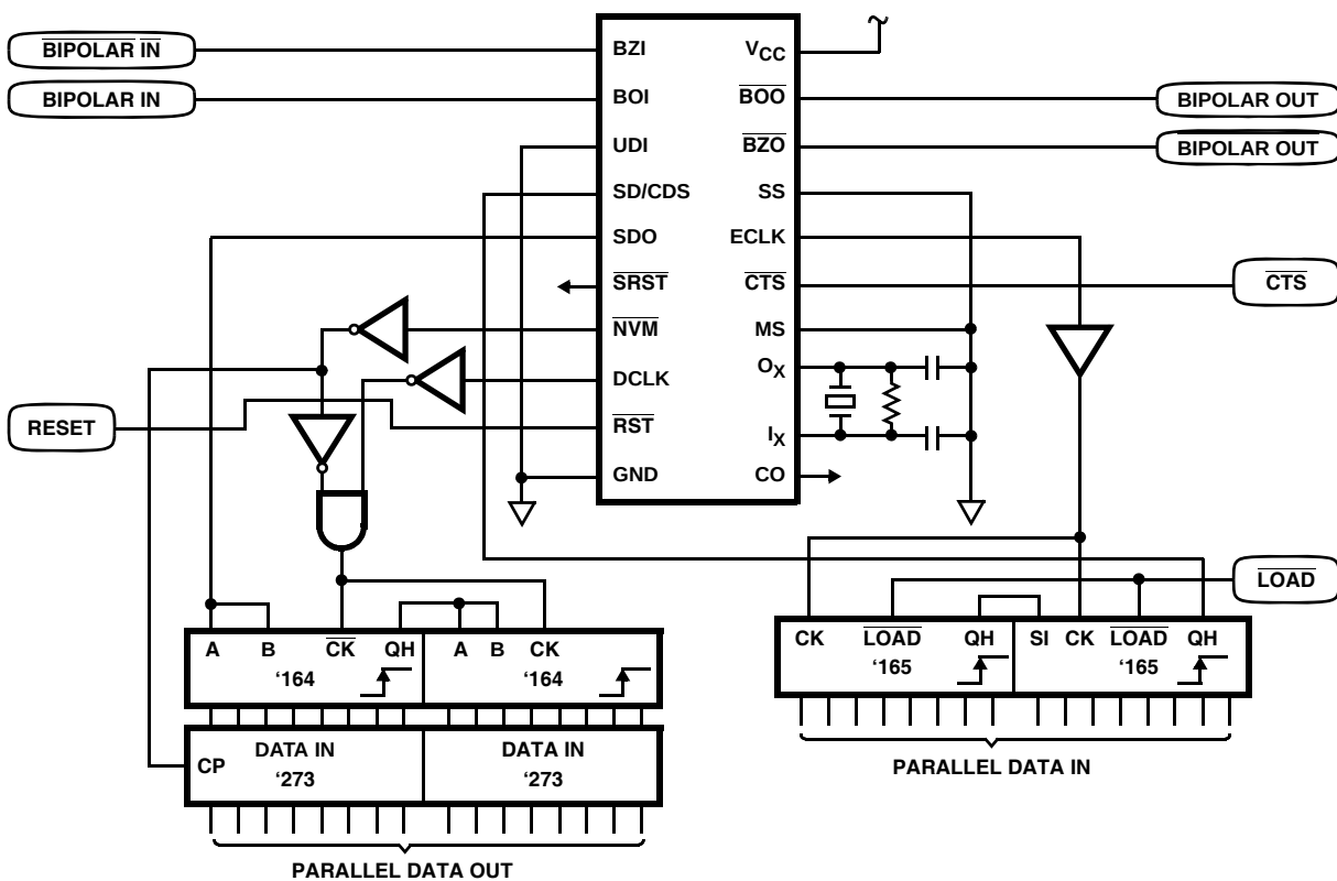
FIGURE 7. MANCHESTER ENCODER UART
