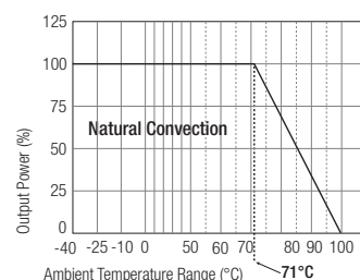
RP30-4805SE With Heat Sink
