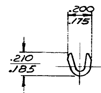
SECT. - A-A
