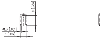
Dimensional drawing
