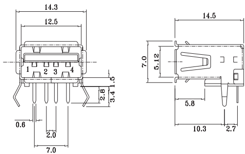
Dimensional drawing
