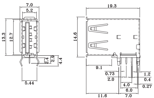
Dimensional drawing
