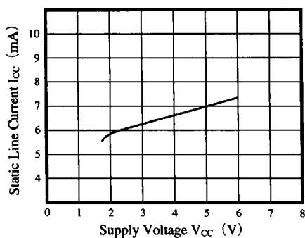
I_{CC}-V_{CC} Characteristics
