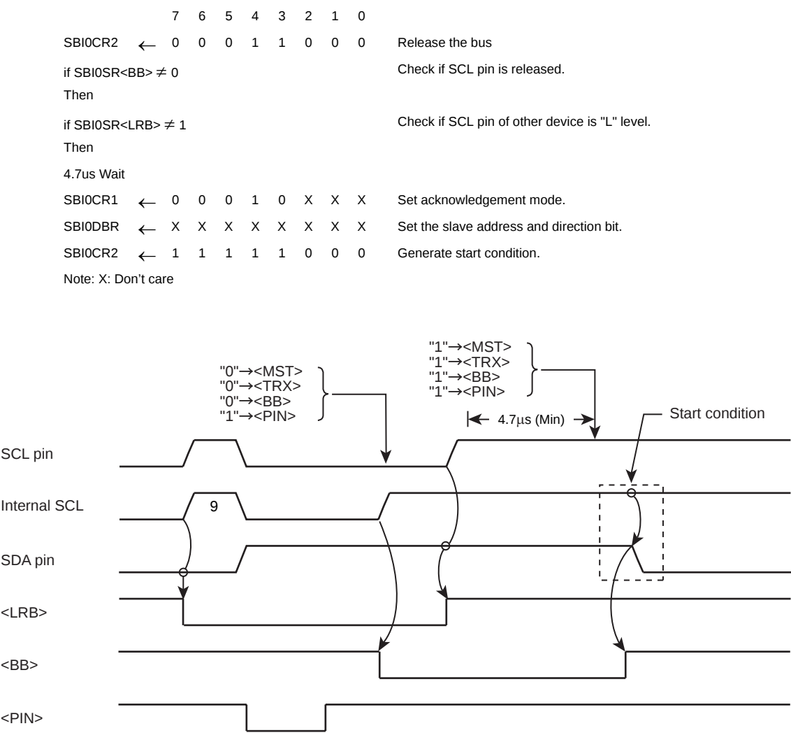
Figure 9-15 Timing Diagram for TMP91FW60 Restart
