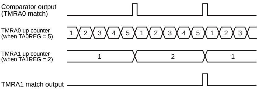
Figure 6-6 TMRA1 Count Up on Signal from TMRA0
