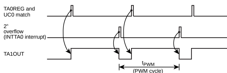
Figure 6-11 8-Bit PWM Waveforms
