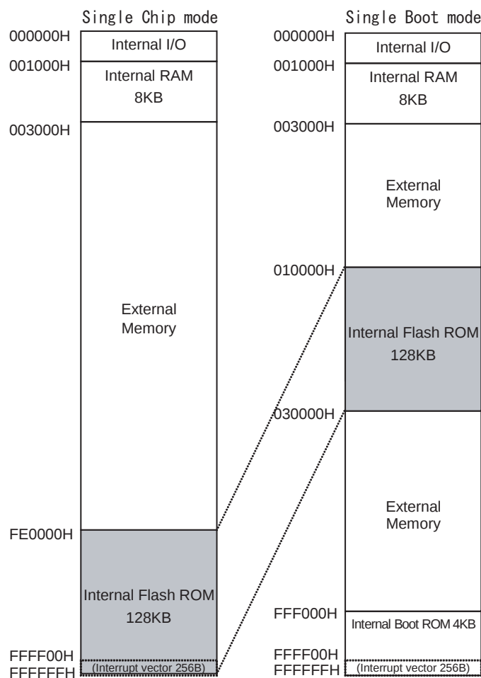
Figure 14-6 Comparison of Memory Maps
