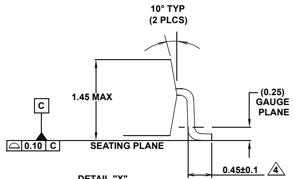
DETAIL "X"
