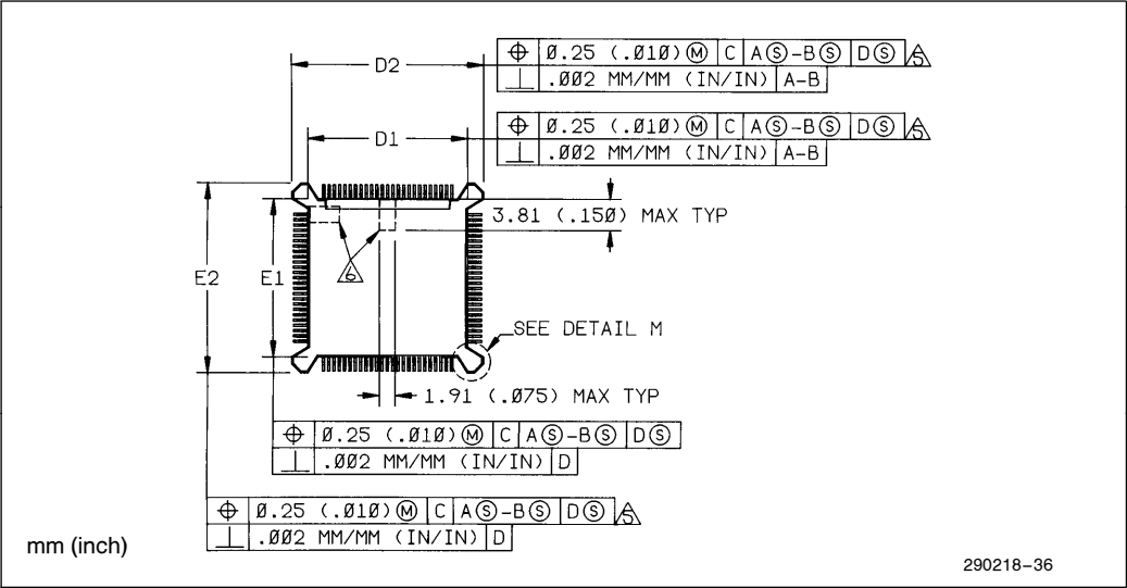
Figure 62. Molded Details
