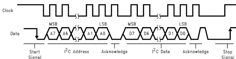
Figure 34. I²C Bus Format
