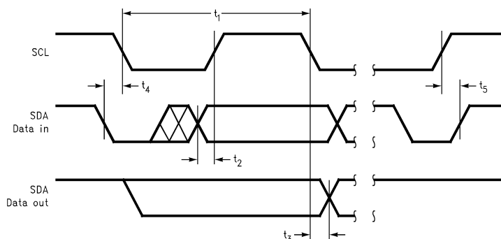
Figure 35. I²C Timing Diagram
