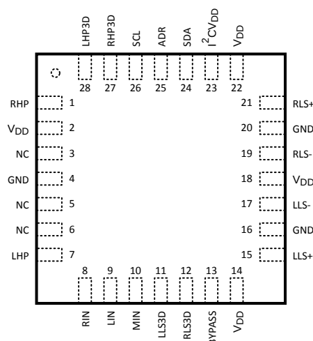
Figure 3. 28 – Lead UQFN Package, Top View See Package Number NJD0028A
