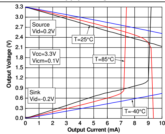
Figure 13. Output characteristics at 3.3 V supply voltage
