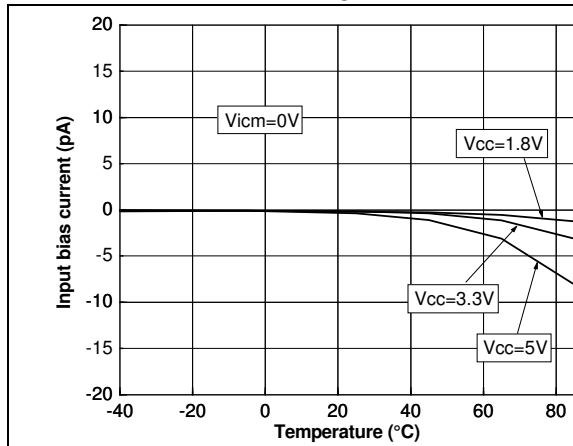
Figure 10. Input bias current vs. temperature at low V_{ICM}
