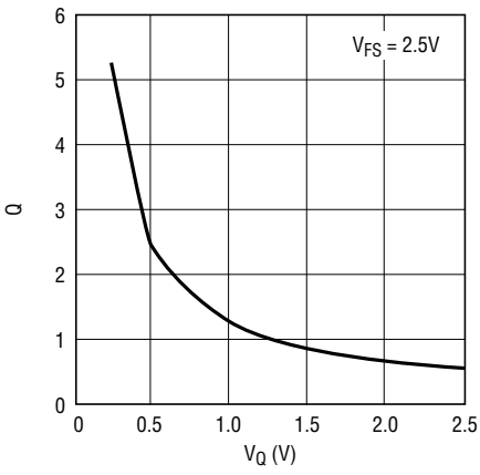
Q vs Control Voltage V_Q
