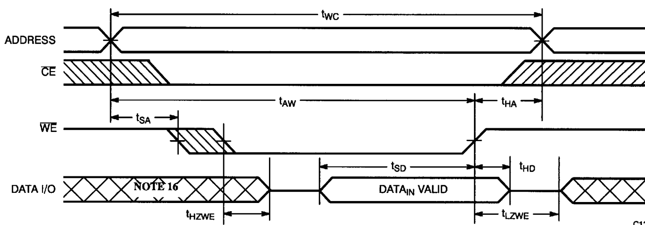
Write Cycle No. 3 ( \overline{WE} Controlled, \overline{OE} LOW)[10, 15]
