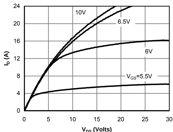
Fig 1: On-Region Characteristics
