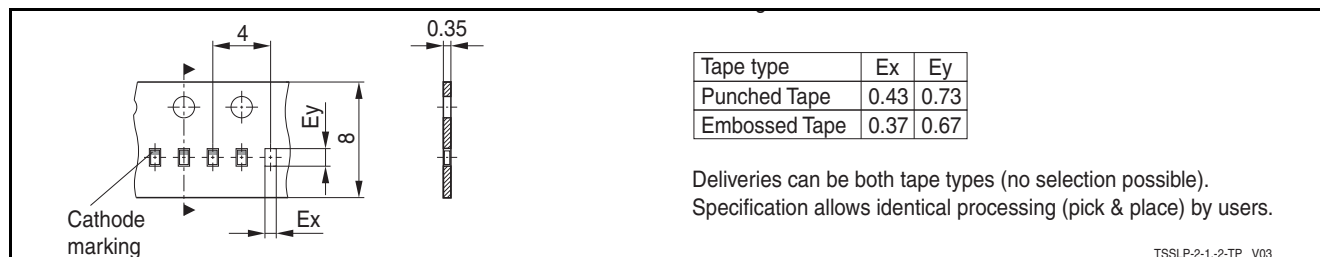
Figure 6-3 PG-TSSLP-2-1: Packing
