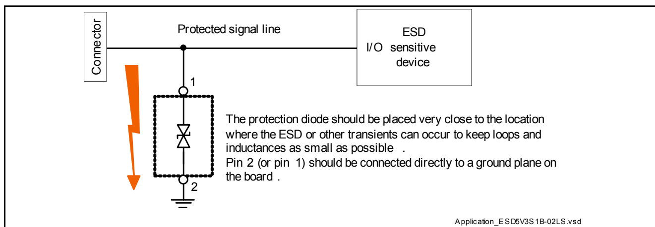
Figure 4-1 Single line, bi-directional ESD / Transient protection
