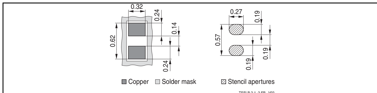
Figure 6-2 PG-TSSLP-2-1: Footprint
