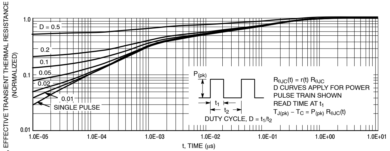
Figure 13. Thermal Response
