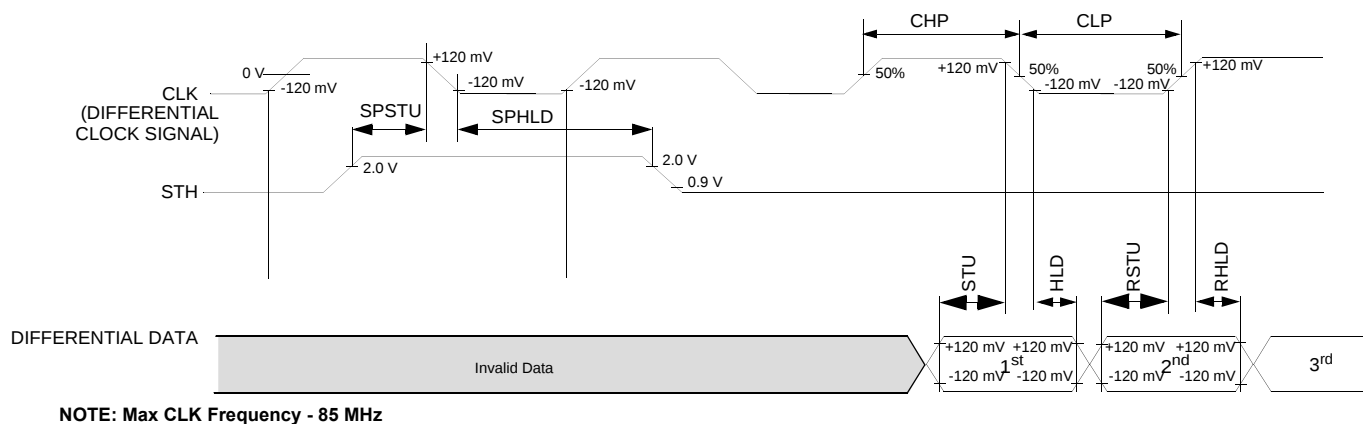
Figure 4. Timing Specifications 1
